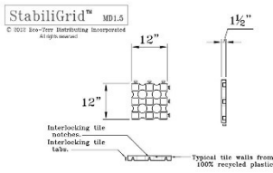
Typical Grid Tile no scale
